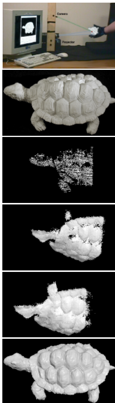
Figure 1: Our real-time 3D model acquisition system was used to scan a small turtle figurine. The total scanning time was 4 minutes and the final model, at 1/2 mm. resolution, contains approximately 200,000 polygons. (c) through (e) are rendered using splats (see Section 2.3), and (f) is rendered as a polygon mesh (see Section 2.4).
